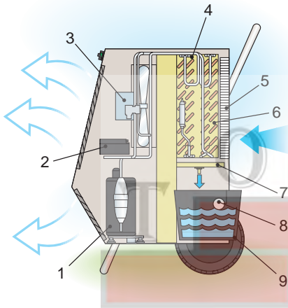
Fig. 1 How the unit works: 1. Air-tight compressor. 2. Control device 3. Helical fan 4. Condenser 5. Air filter 6. Evaporator 7. Tube fitting 8. Float 9. Water tank (Except DH 80).
